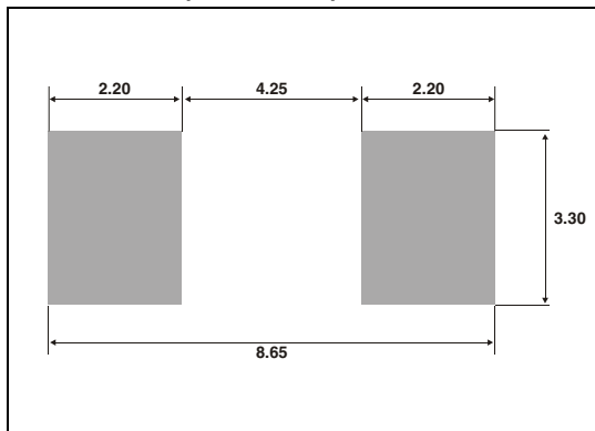
Figure 9. Footprint dimensions (millimeter)
