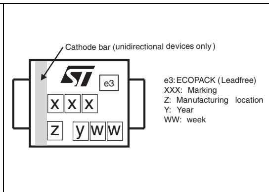
Figure 10. Marking layout
